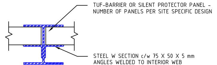
TYPICAL CROSS SECTION "B-B" SCALE: N.T.S. REF: SW-SE-050
