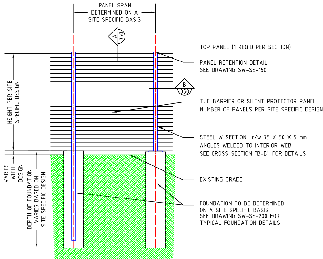
TYPICAL ASSEMBLY ELEVATION VARIES WITH DESIGN HEIGHT SCALE: N.T.S. REF: NONE
