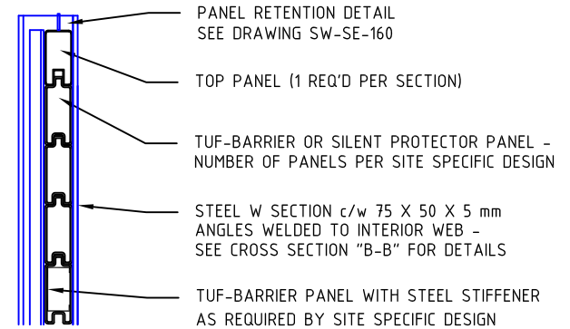
TYPICAL CROSS SECTION "A-A" SCALE: N.T.S. REF: SW-SE-050
